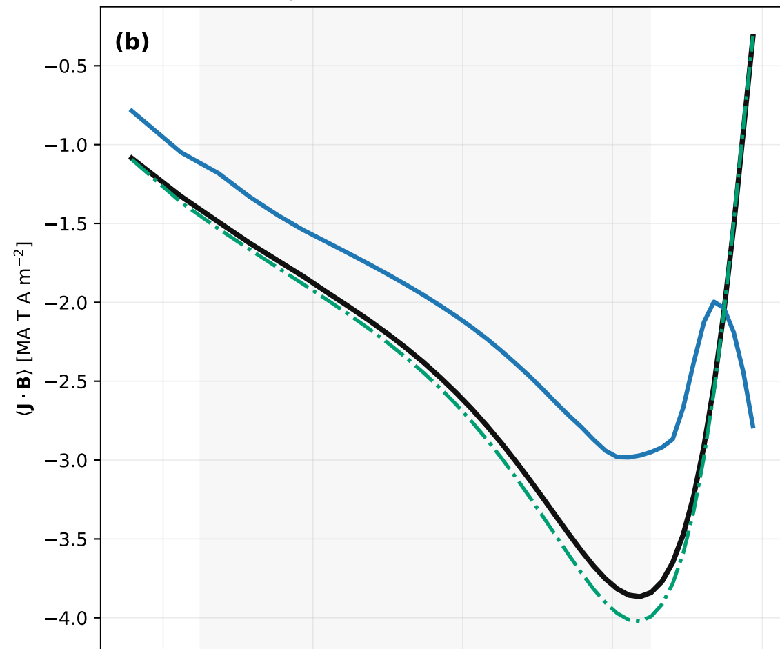
QH precise-QS fixed-field reference
