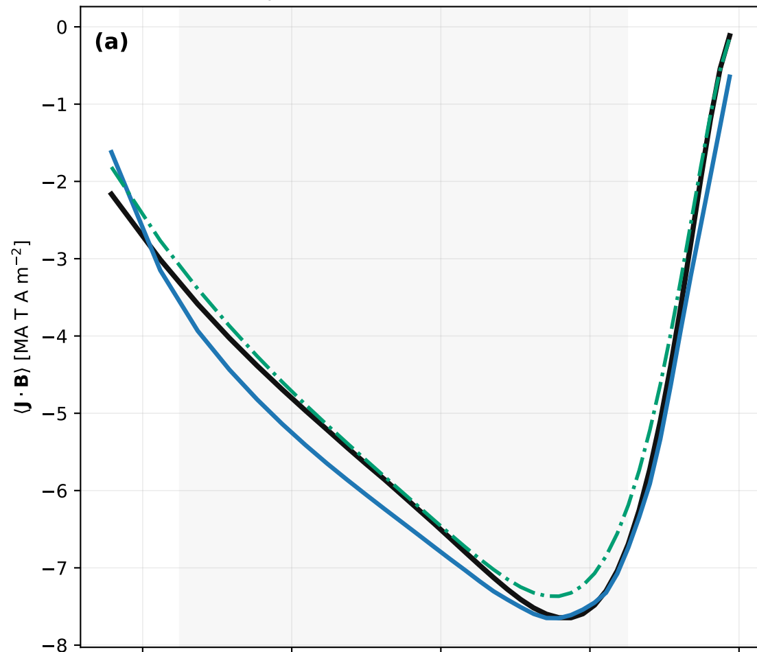
QA precise-QS fixed-field reference
