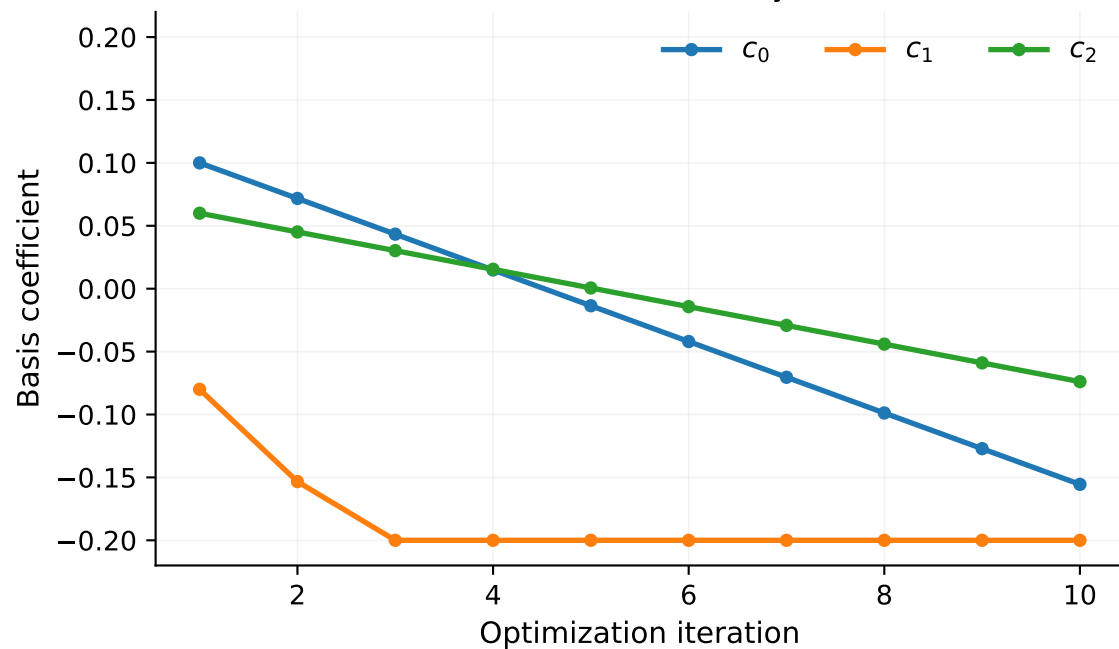
Optimized ambipolar field
