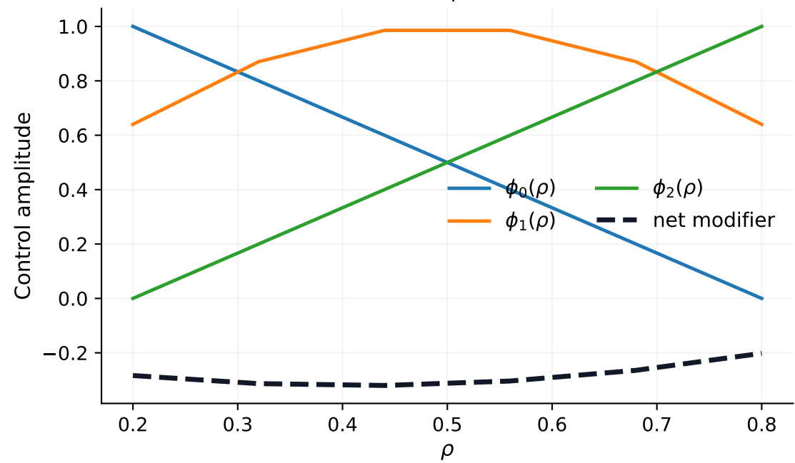
Optimized current profile
