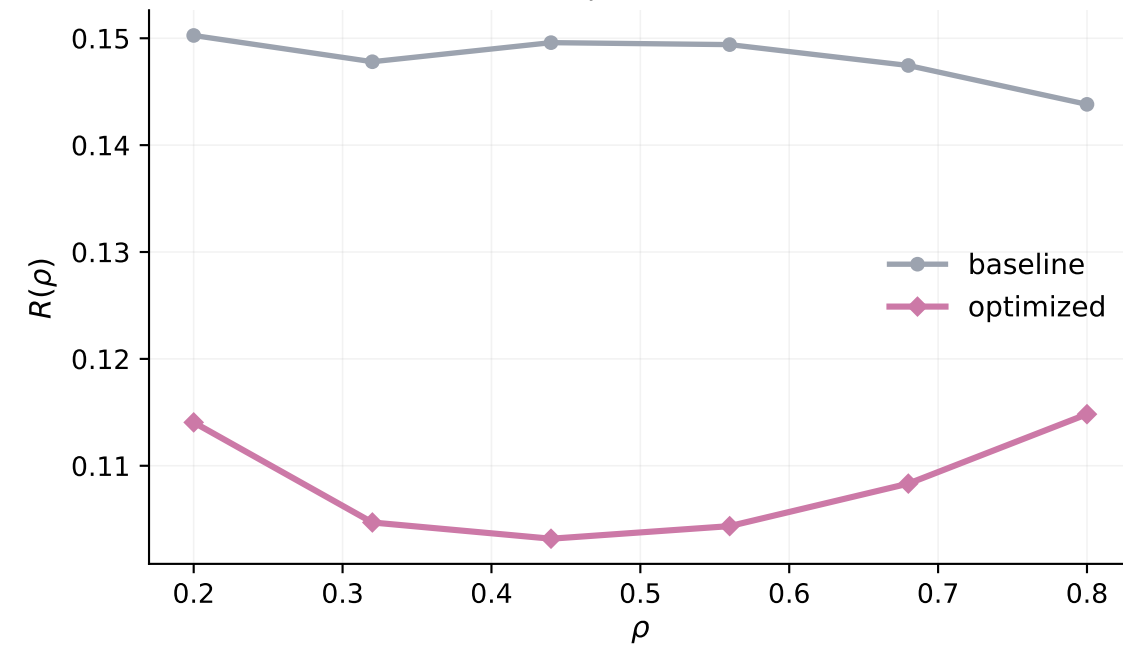
Residual-profile reduction
