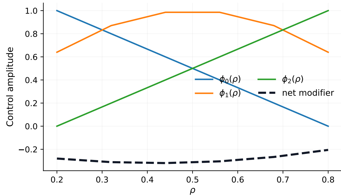
Optimized current profile
