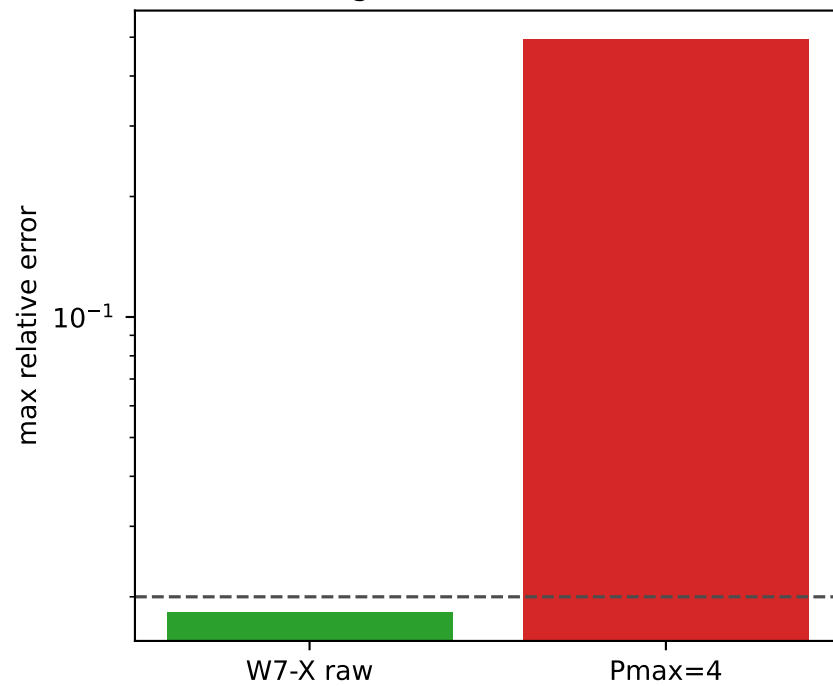
Integrated W7-X transfer
