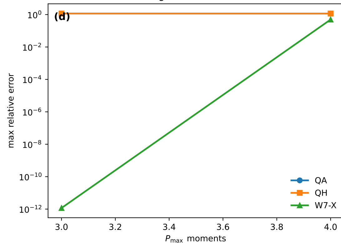
Higher-order stress
