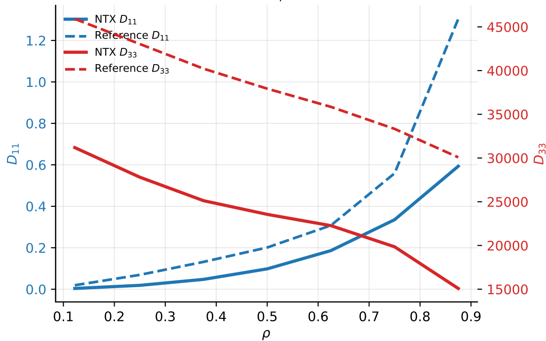
Radial Coefficient Comparison
