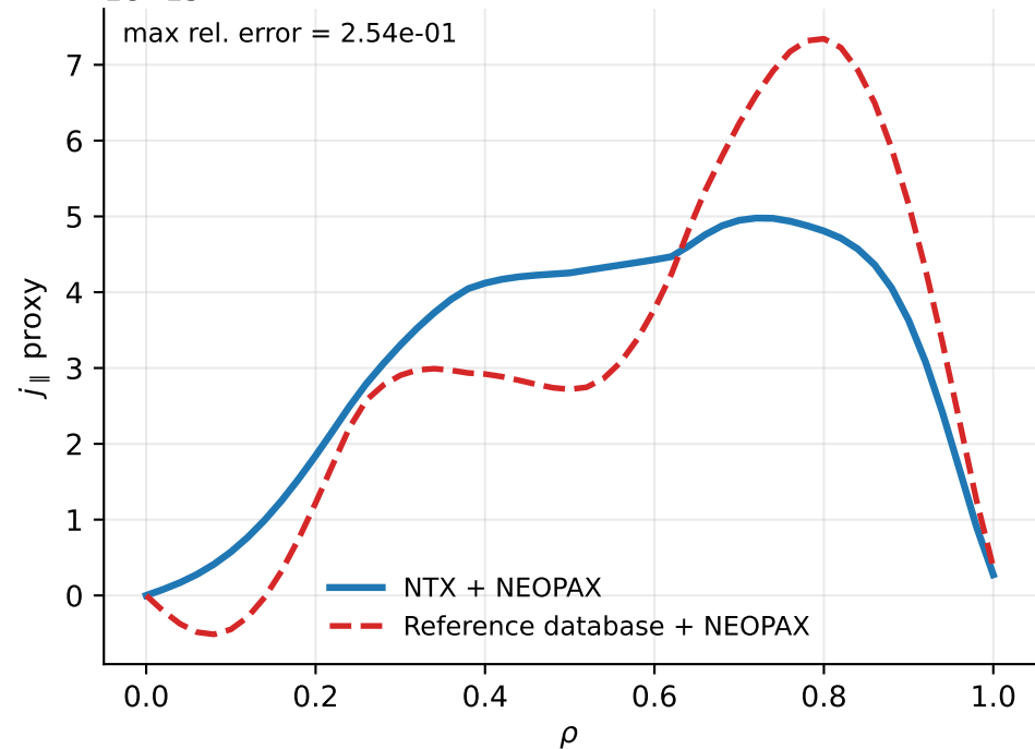
b Bootstrap-Current Profile
