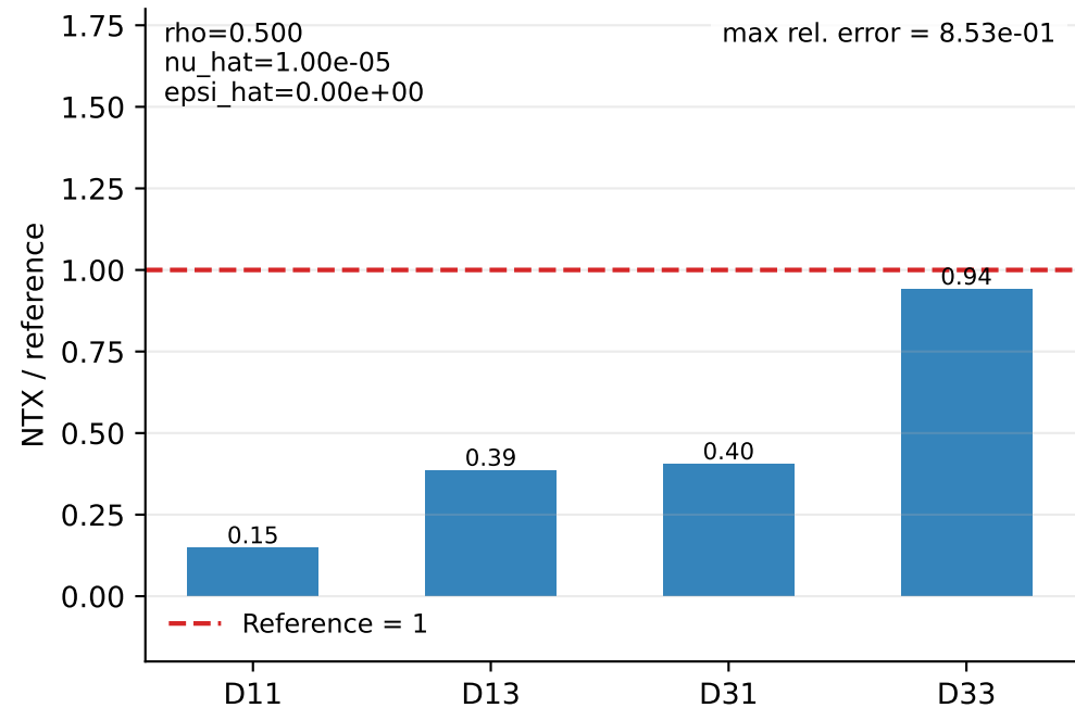
a Pointwise Coefficient Ratios at \rho = 0.50
