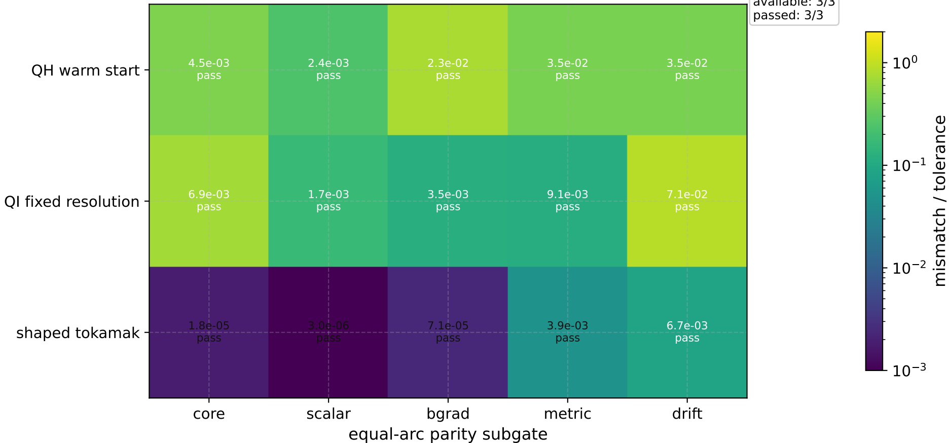
VMEC/Boozer equal-arc parity matrix at mboz=nboz=21
