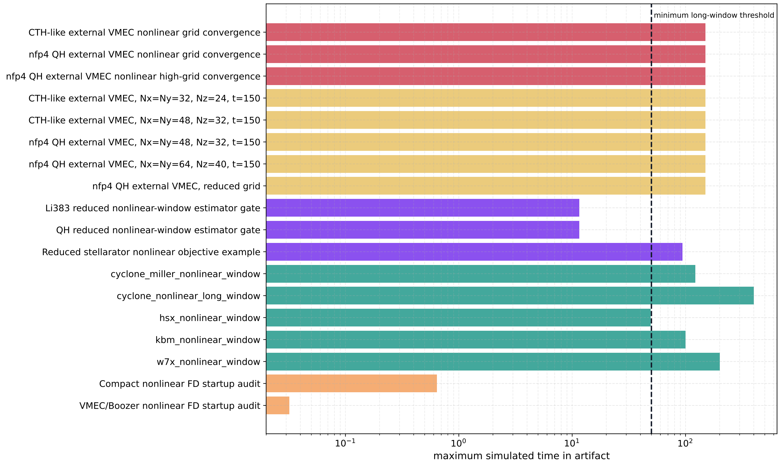
Nonlinear heat-flux artifact time-horizon audit
