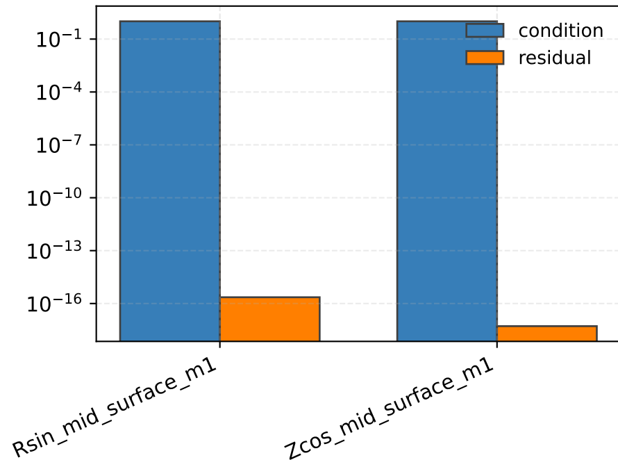
Mapping quality
