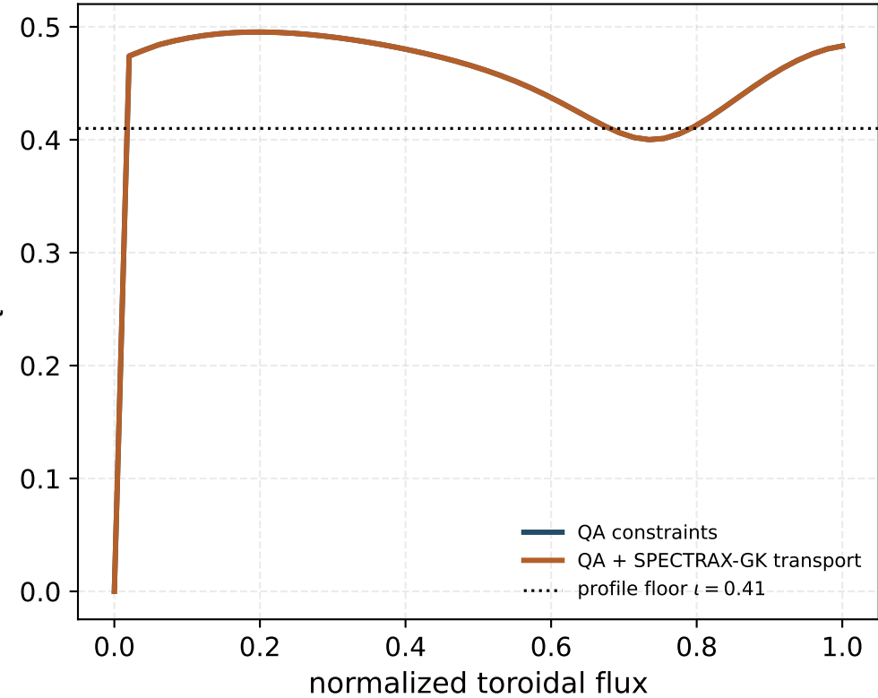
Final WOUT iota profiles
