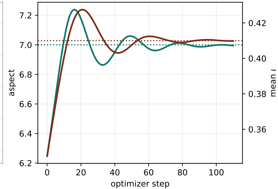
QA constraints
