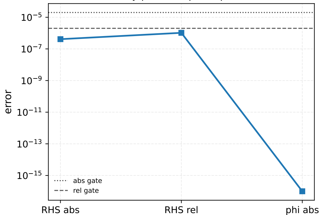
Identity passed; speedup=0.04x
