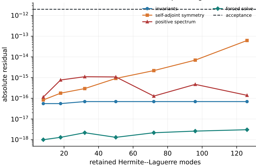
(c) Conservation and dissipation gates
