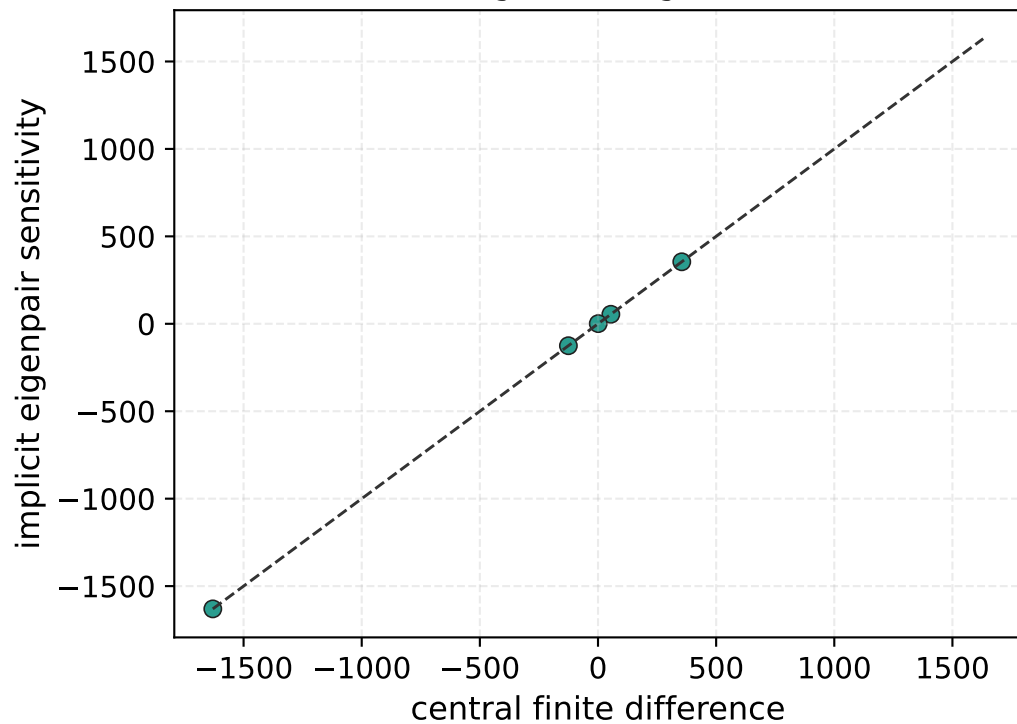
AD/FD gradient agreement
