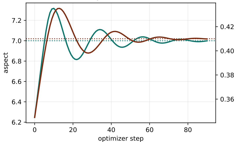
QA constraints
