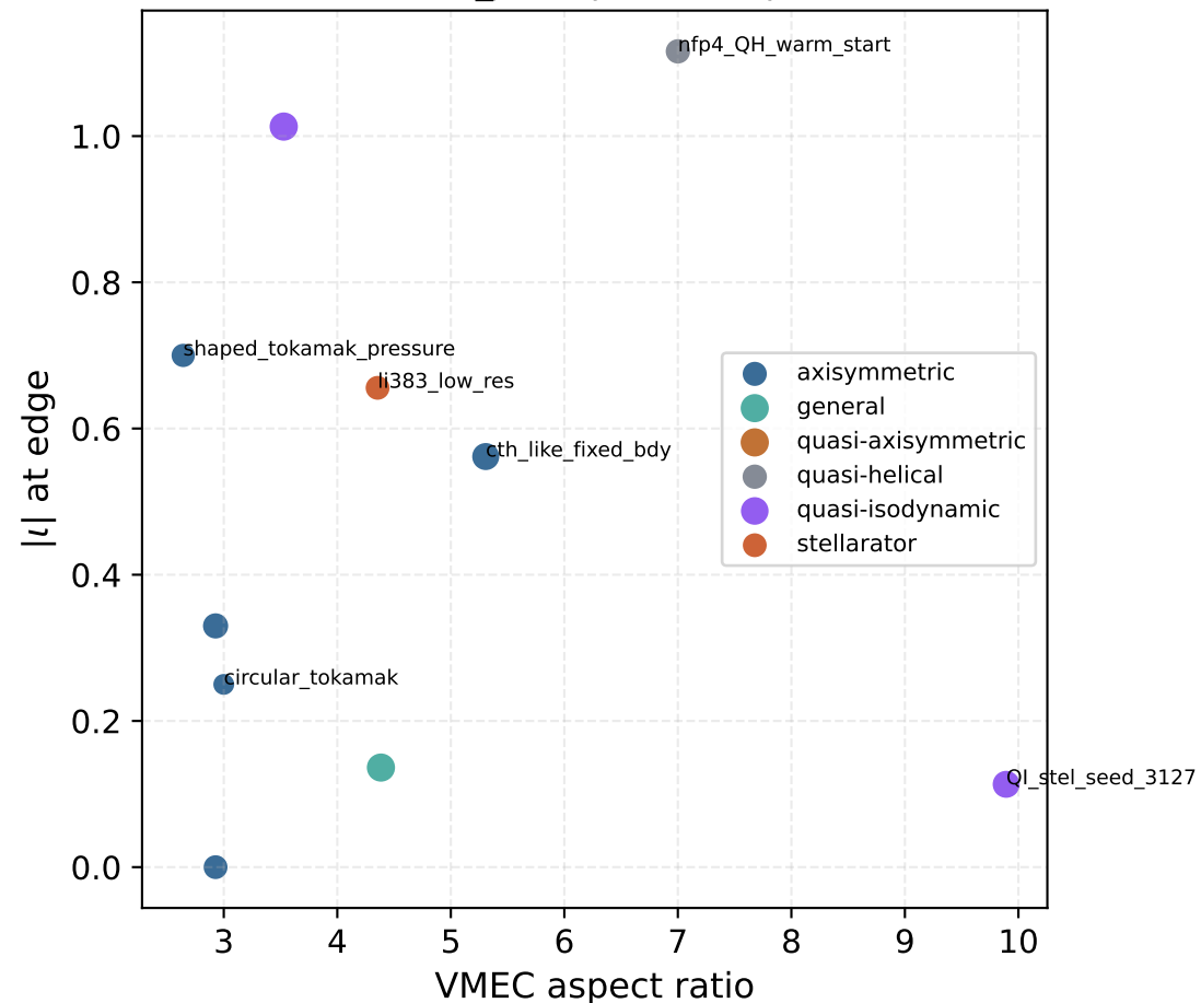
Local vmec_jax equilibrium portfolio
