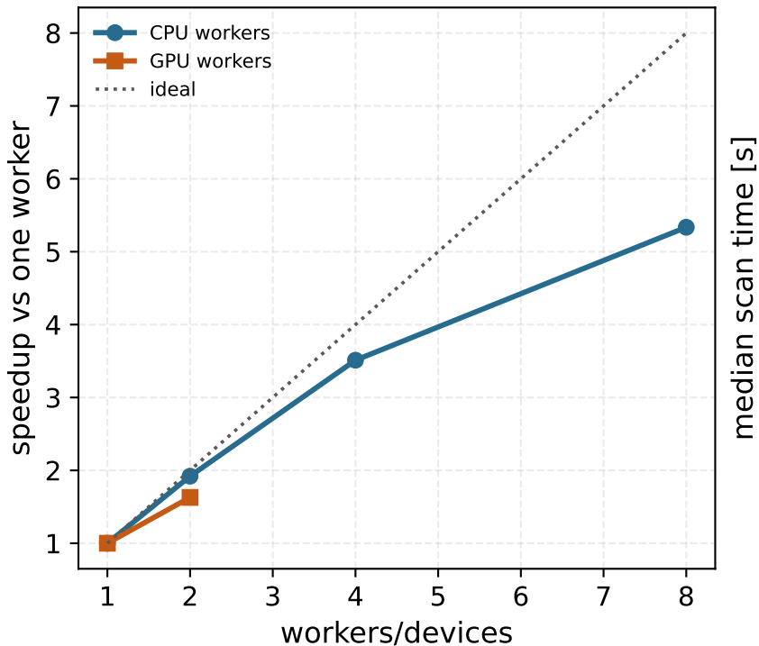
Independent ky strong scaling
