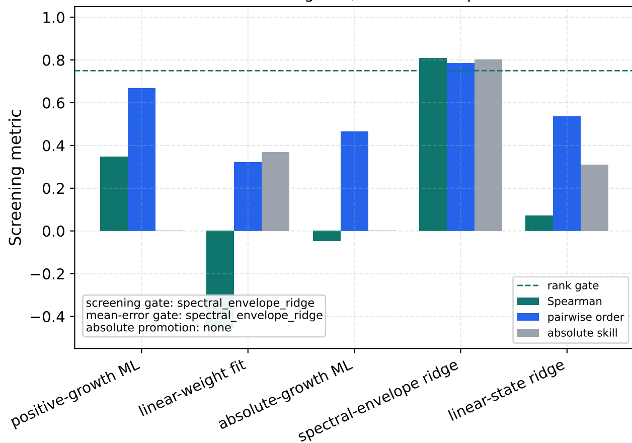
Correlation/ranking skill, not absolute promotion
