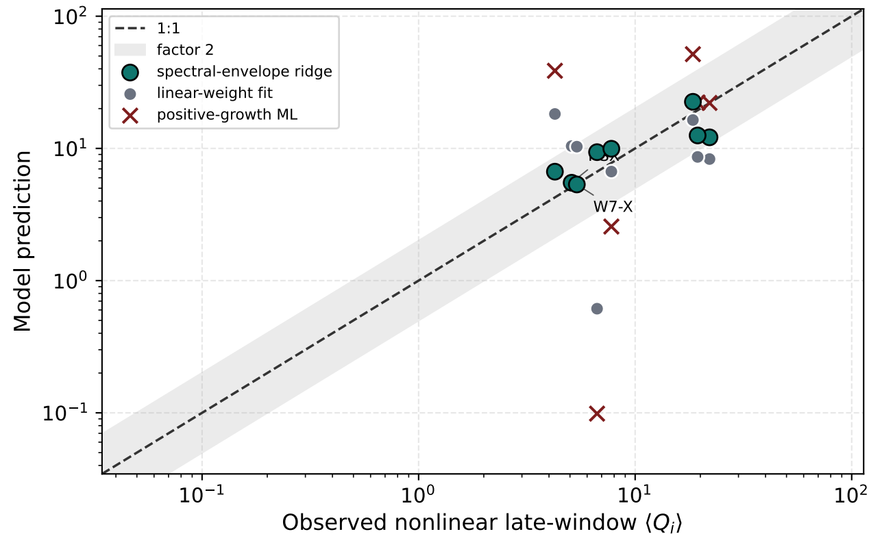
Best screened model vs nonlinear windows
