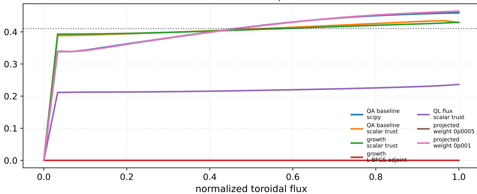
Solved WOUT iota profiles
