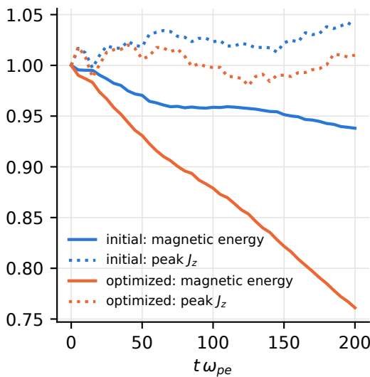
ane magnetic energy and peak J_z , relative to t = 0
