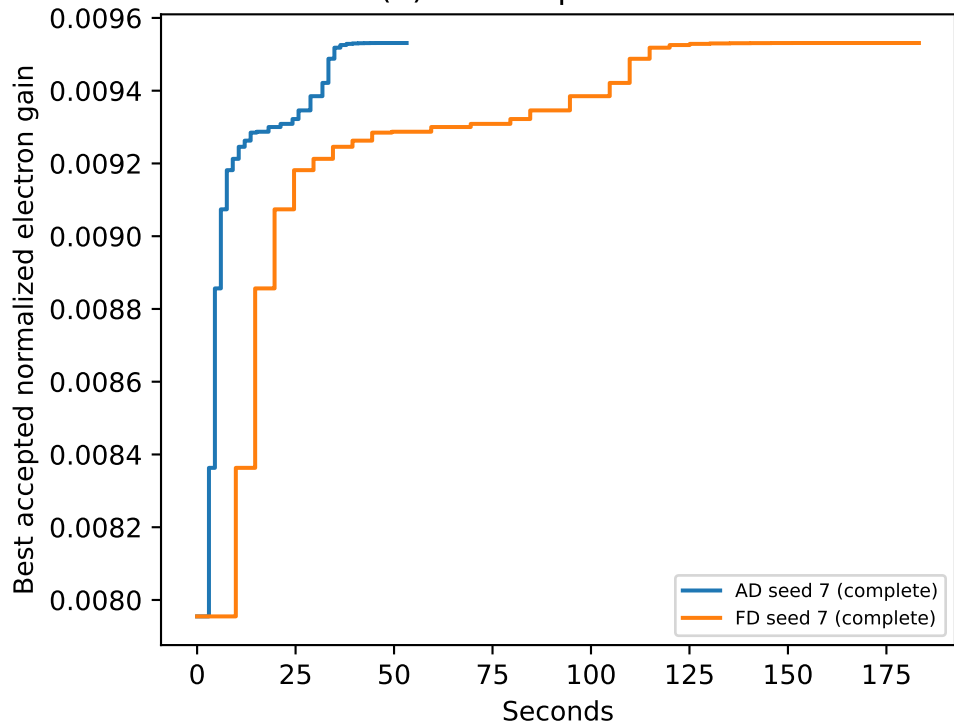
(b) Warm optimization
