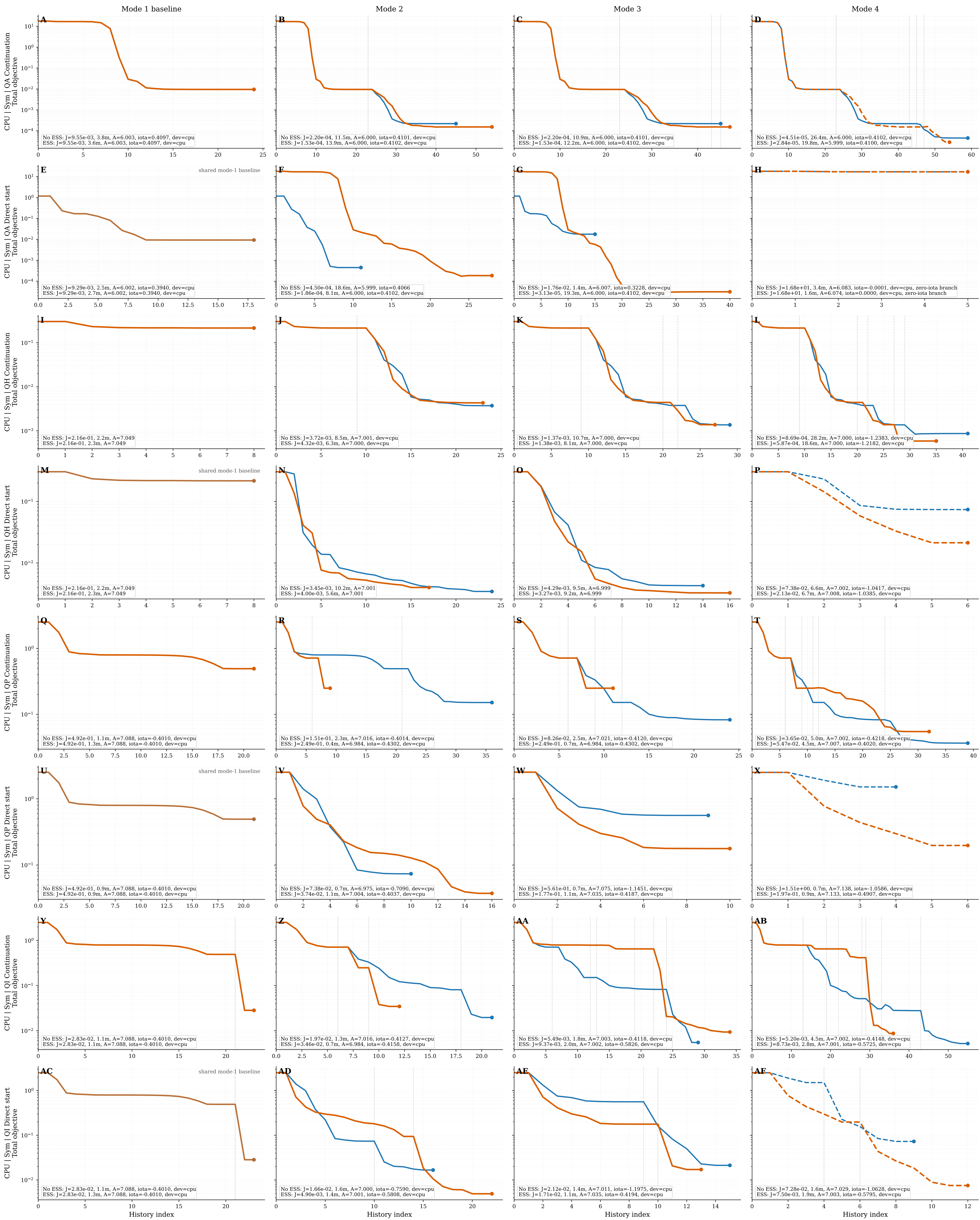
QA/QH/QP/QI optimization histories by backend and boundary symmetry
