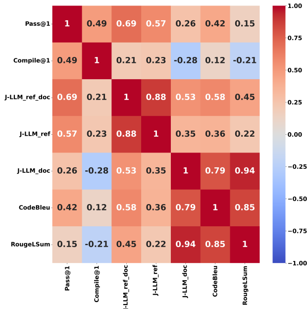
FIGURE 4: The correlation matrix of different metrics, including pass@1, compile@1, three different J-LLM instances, and the similarity scores CodeBLEU and ROUGE-LSUM.
