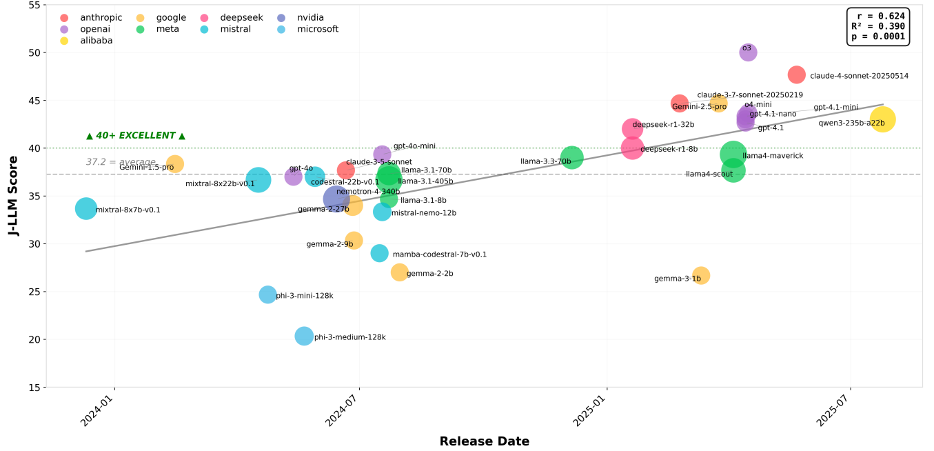
FIGURE 3: Temporal evolution of S-LLM performance on SimBench. Y-axis is the average of three modalities of J-LLM scores, they are plotted against model release dates, showing a positive trend ( \rho = 0.624 , p < 0.001 ).
