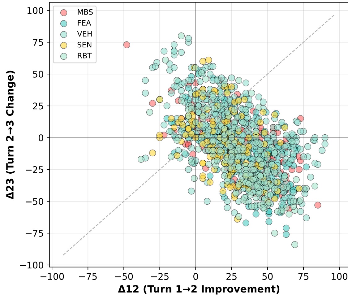
Delta Correlation
