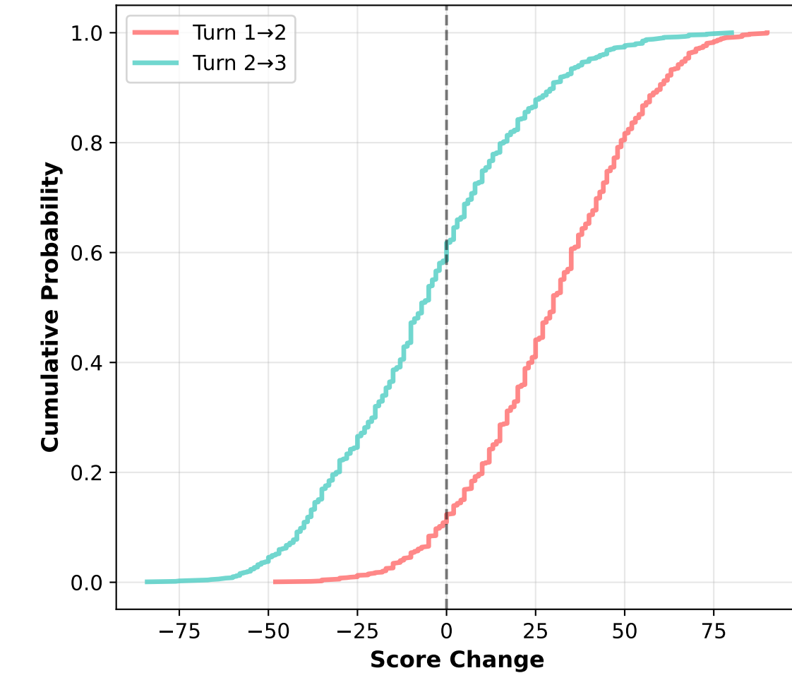
Cumulative Distribution
