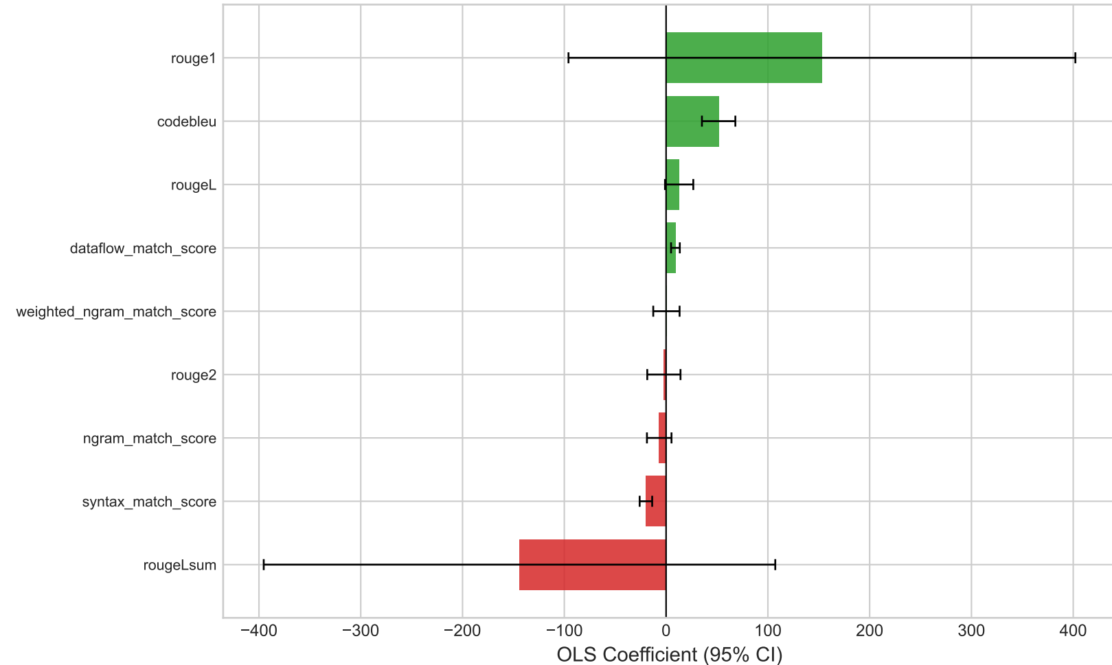
Regression Coefficients (Predicting J-LLM from CodeBLEU/ROUGE)
