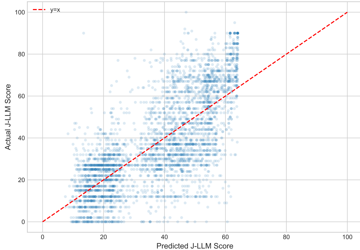
Regression: Actual vs Predicted ( R^2=0.516 )
