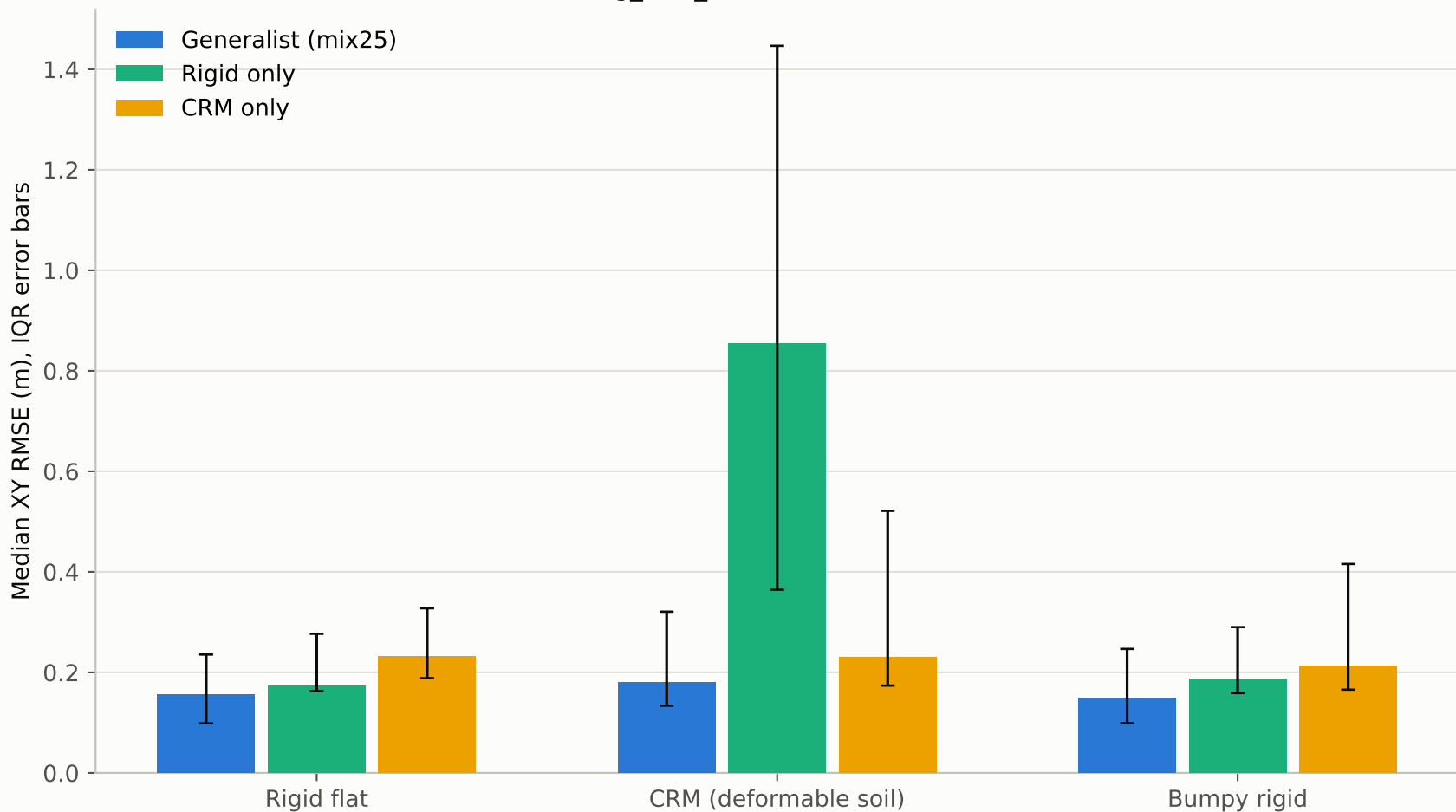
OFAT L8 dynamics backbone: Chrono tracking, median XY RMSE by policy \times terrain (steering_rate_limit=0.1, 20 rollouts/cell)
