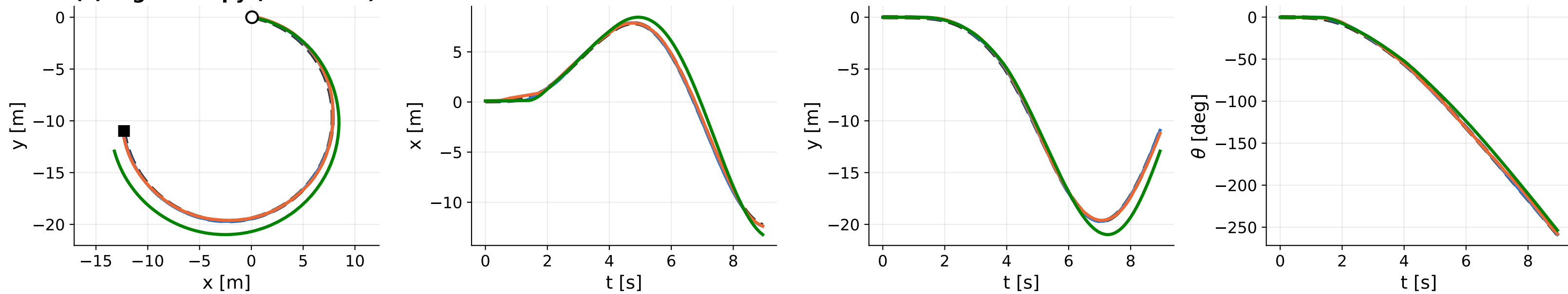
(c) Rigid bumpy (zero-shot)
