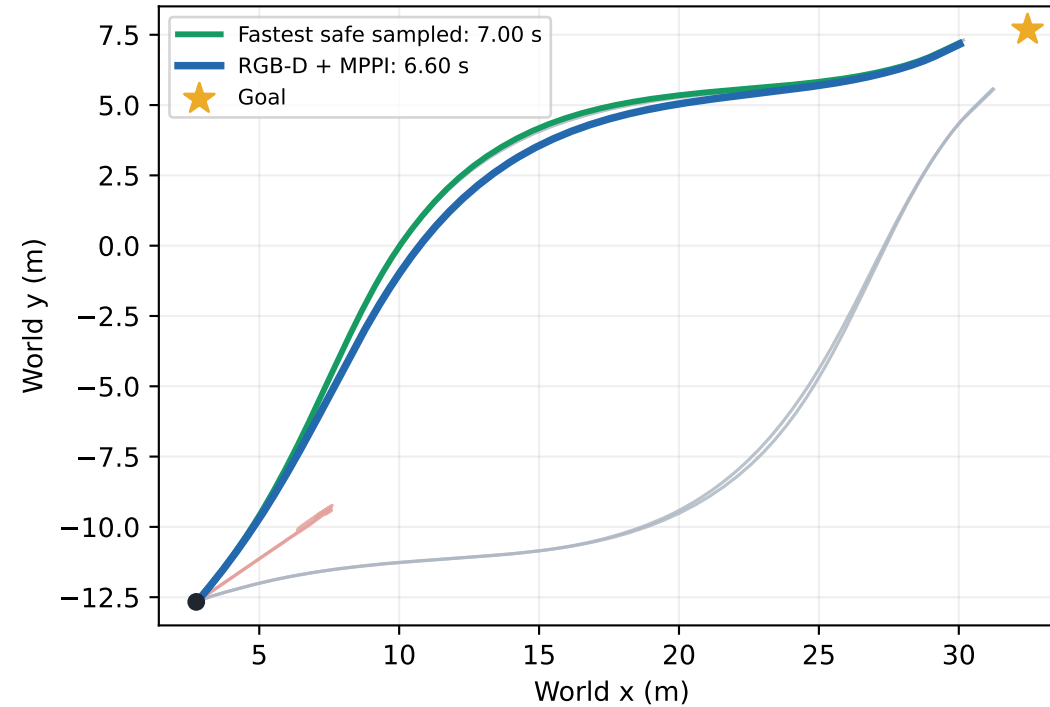
Safe goal reached — actual Chrono paths
