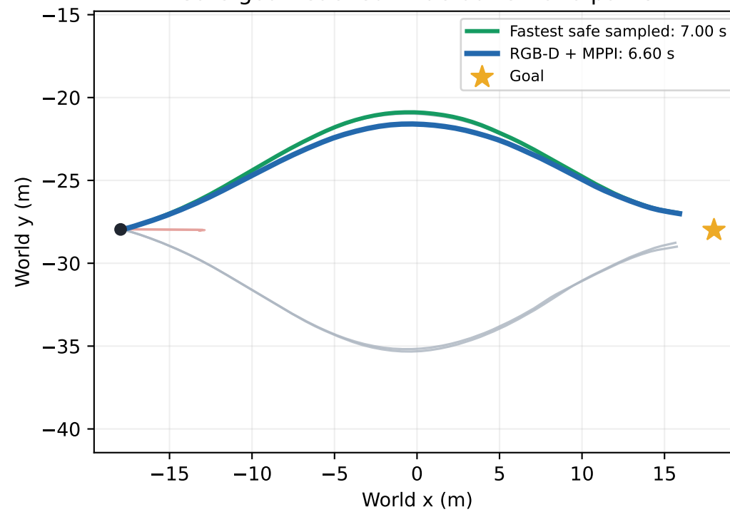
Safe goal reached — actual Chrono paths
