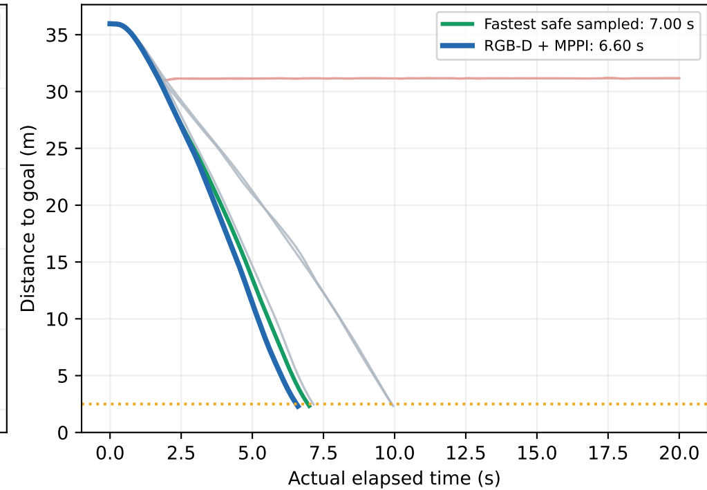
Measured goal progress
