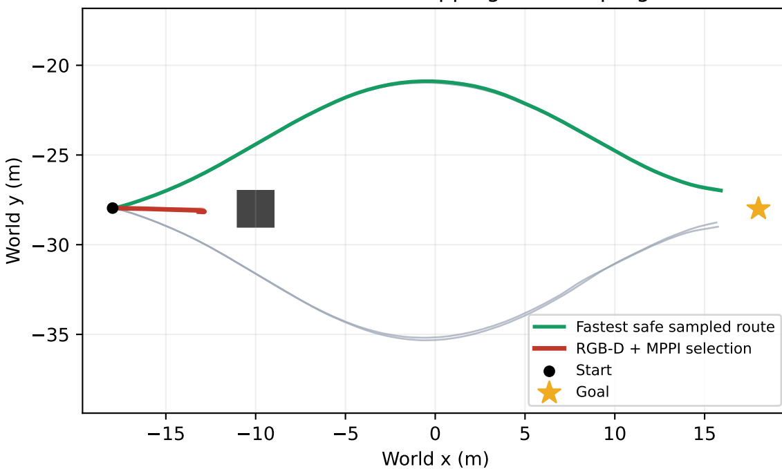
Visible obstacle FAILED: contact and stopping; 4.81 m progress
