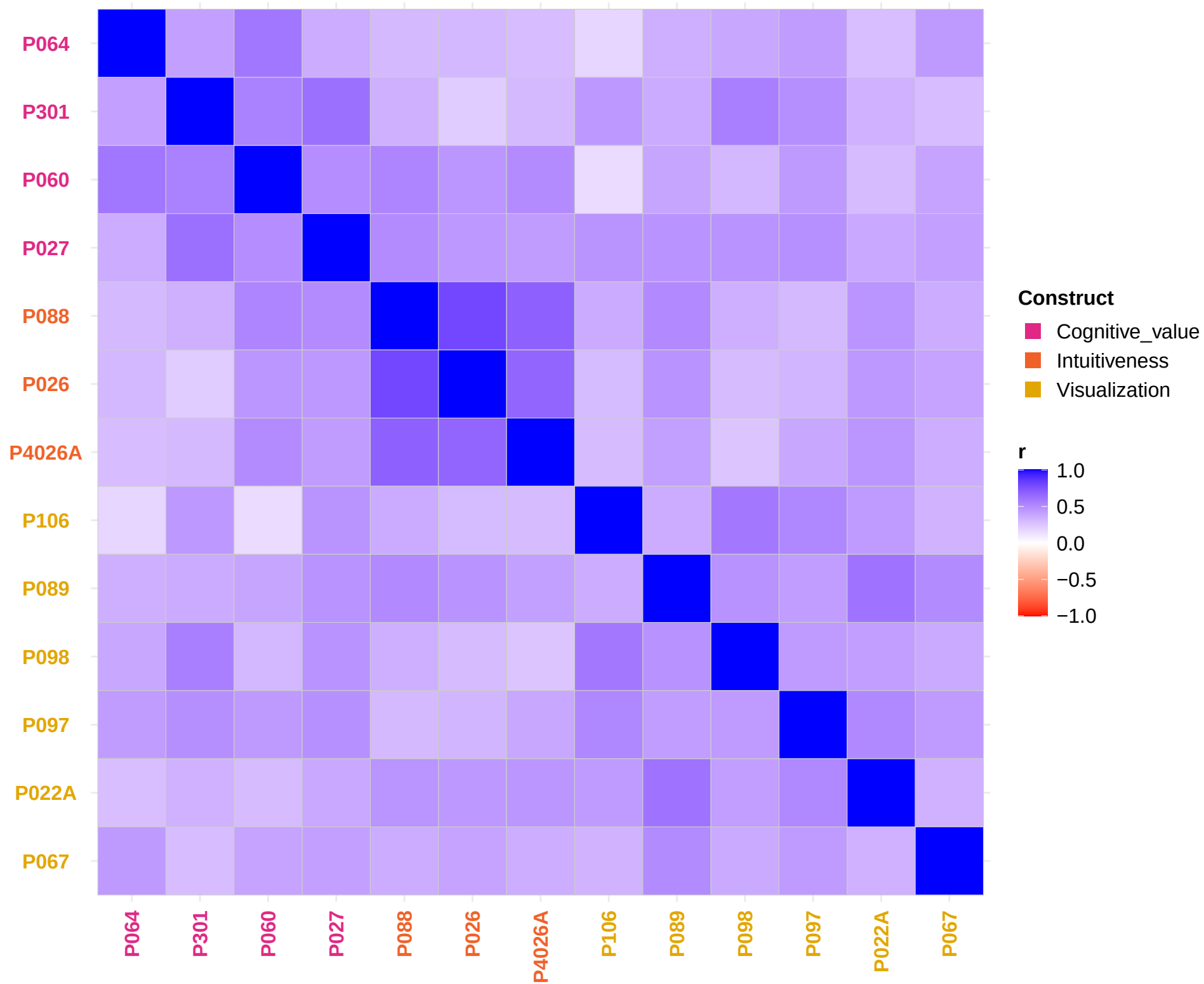
Polychoric correlations, ordered by construct
