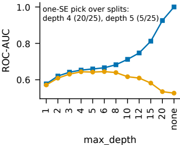
pre-pruning
