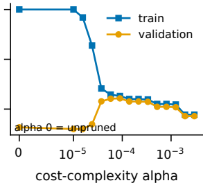
post-pruning
