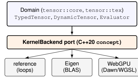
Figure 1: Hexagonal-lite kernel backend: one port (orange), three concrete adapters (grey). The Domain knows only the port; the static_assert(KernelBackend<Backend>) at the end of each adapter file enforces conformance at the adapter’s own compile site.
