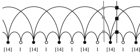
Figure 4: The juggling diagram of the multiplex juggling sequence [14]1. Source: [5, p.66]
