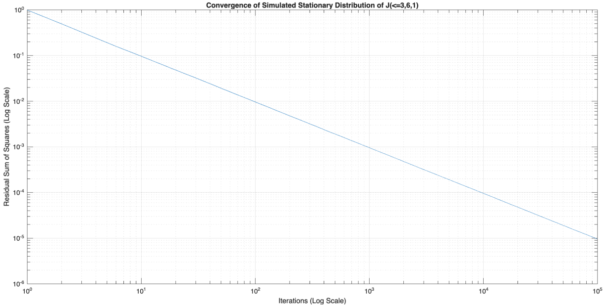
Figure 22: Residual sum of squares plotted against number of iterations to show convergence of simulated stationary distribution with theoretical stationary state for juggling system J(\leq 3, 6, 1) plotted on a log-log plot
