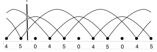
Figure 5: Juggling diagram of a juggling sequence 450 where a ball can be added or dropped. Source: [3, p.9]
