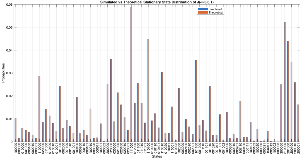
Figure 23: Comparison of the probabilities of simulated stationary state (blue) against theoretical stationary state (red) for juggling system J(\leq 3, 6, 1)
