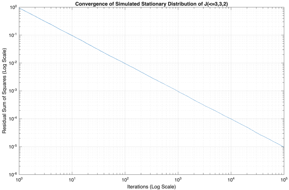
Figure 17: Residual sum of squares plotted against number of iterations to show convergence of simulated stationary distribution with theoretical stationary state for juggling system J(\leq 3, 3, 2) plotted on a log-log plot
