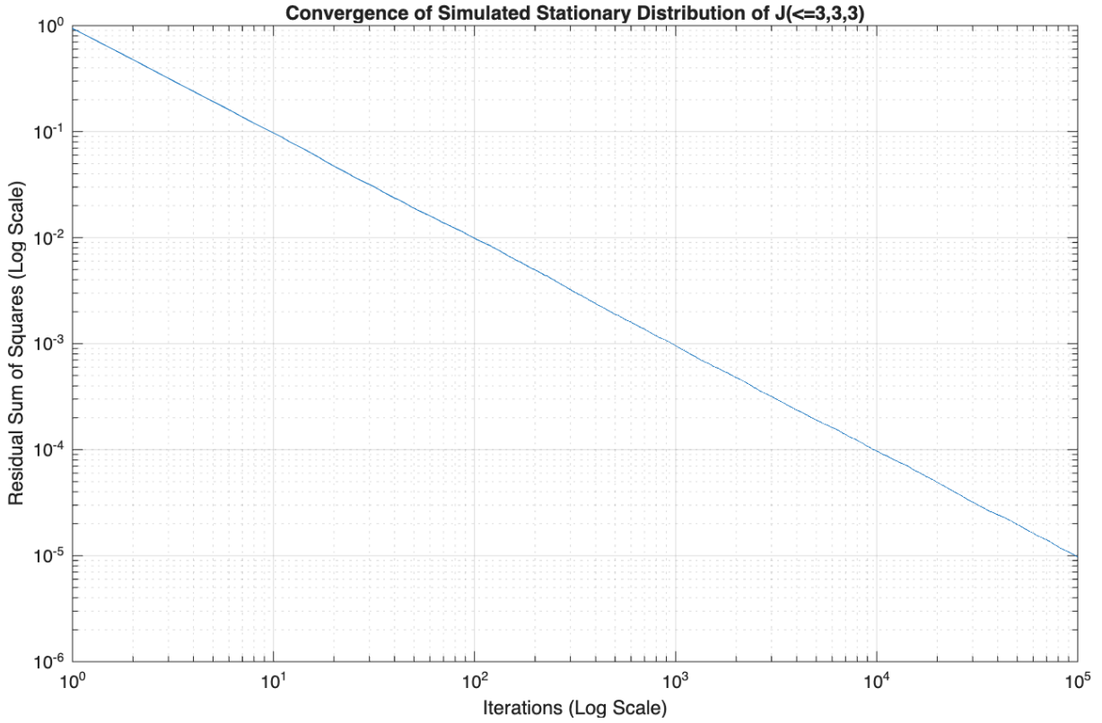
Figure 20: Residual sum of squares plotted against number of iterations to show convergence of simulated stationary distribution with theoretical stationary state for juggling system J(\leq 3, 3, 3) plotted on a log-log plot
