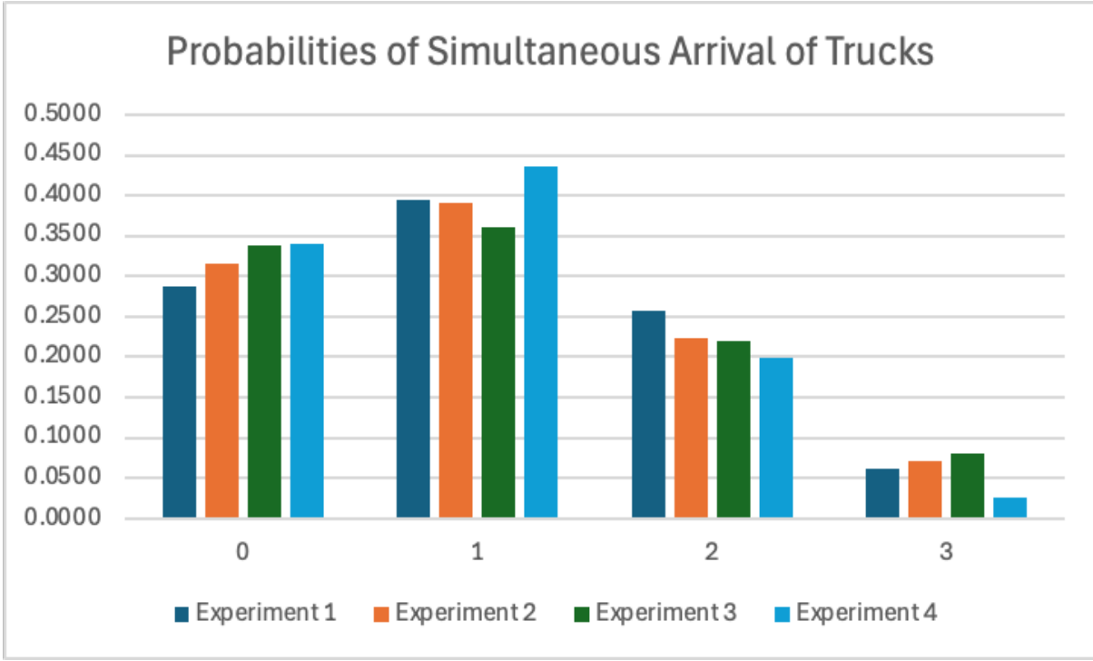
Figure 14: Probability of k trucks arriving simultaneously at the hub for k \in \{0, 1, 2, 3\} , under each of the four experiments. The probabilities are calculated by summing the probabilities of each state starting with k for each experiment.
