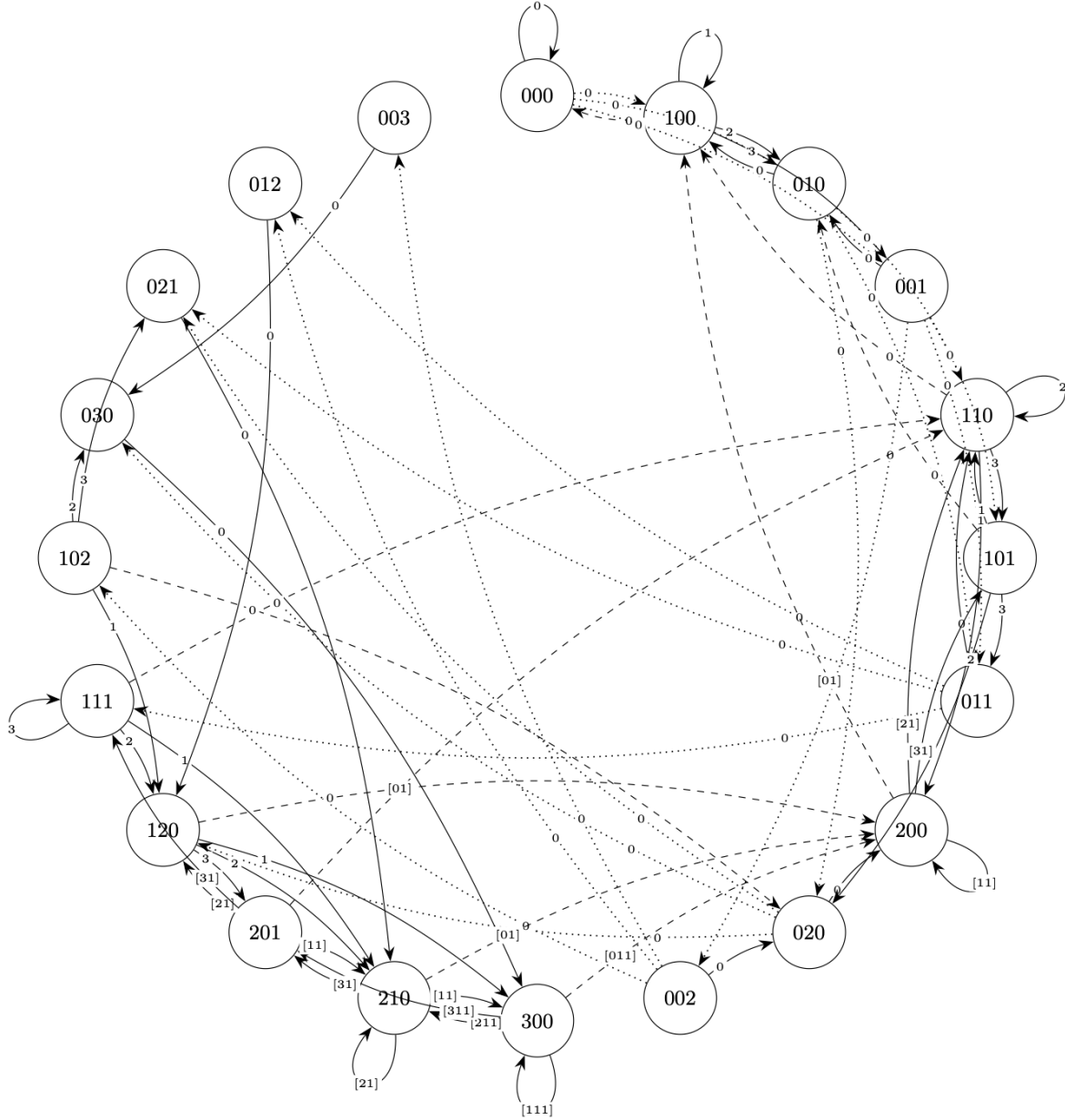
Figure 12: Juggling state graph of up to 3 trucks that can travel for a maximum of 3 hours between the hub with 1 unloading bay and spoke for J(\leq 3, 3, 1) . Source: [18]
