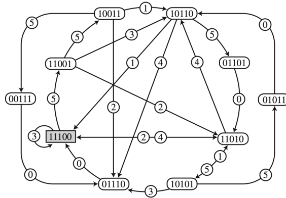
Figure 11: The simple 3 ball juggling state graph of height 5. Source: [5, p.45]
