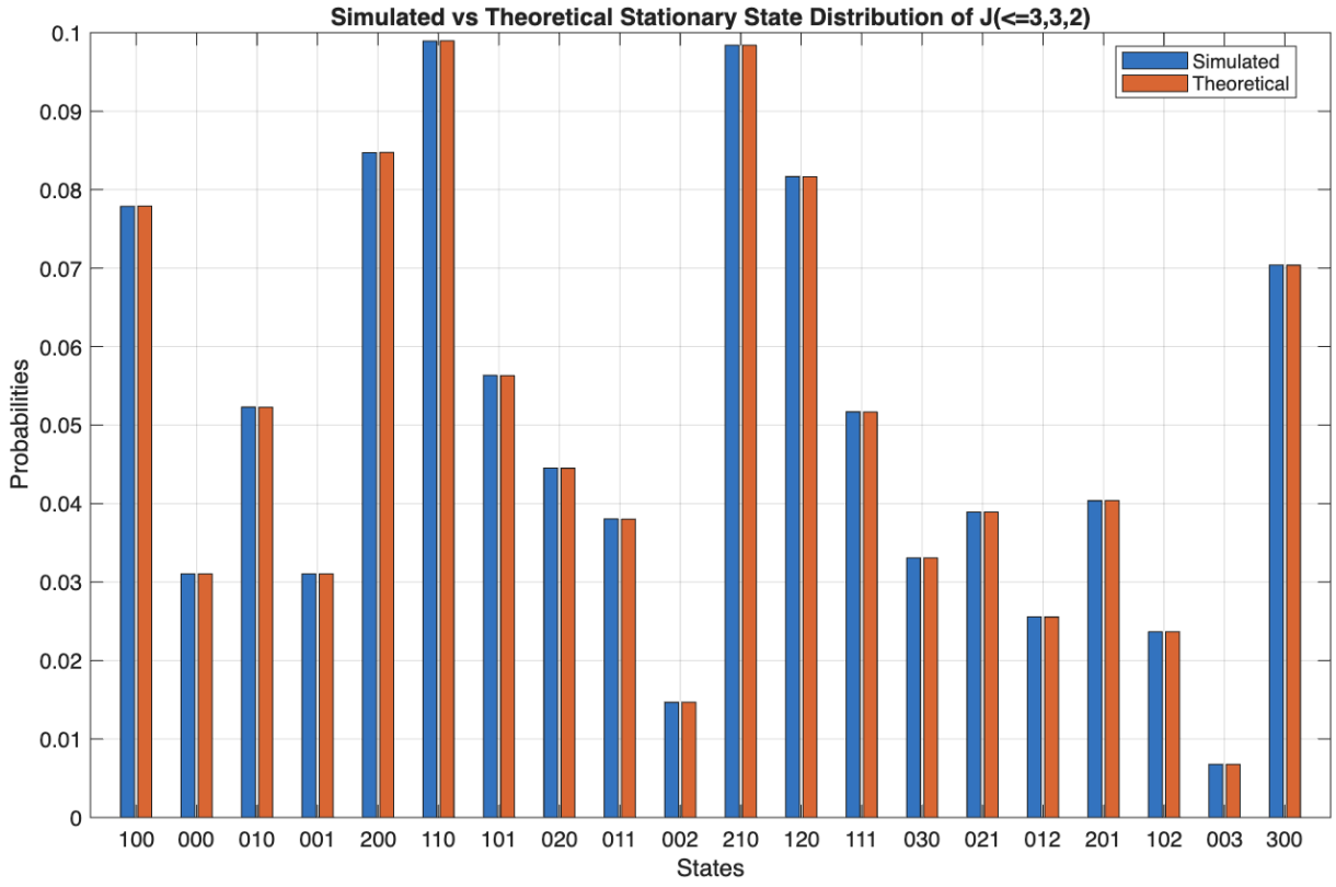
Figure 19: Comparison of the probabilities of simulated stationary state (blue) against theoretical stationary state (red) for juggling system J(\leq 3, 3, 2)
