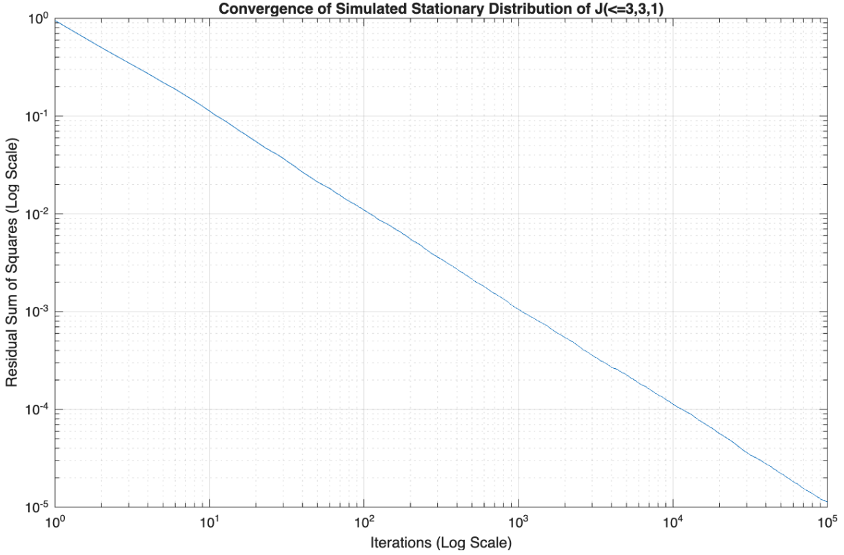
Figure 13: Residual sum of squares plotted against number of iterations to show convergence of simulated stationary distribution with theoretical stationary state for juggling system J(\leq 3, 3, 1) plotted on a log-log plot
