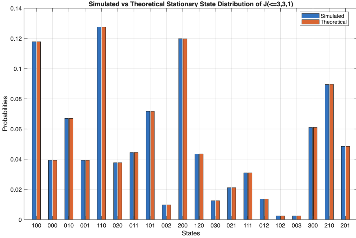
Figure 18: Comparison of the probabilities of simulated stationary state (blue) against theoretical stationary state (red) for juggling system J(\leq 3, 3, 1)
