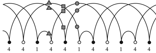
Figure 3: Juggling diagram of juggling pattern 441. Source: [5, p.46]
