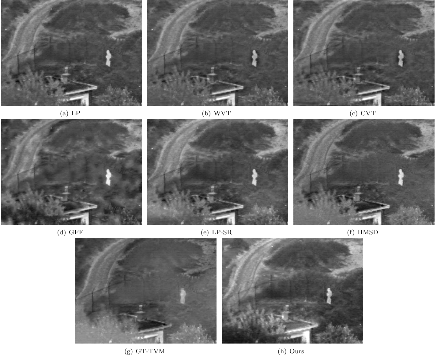
Figure 1: Comparison on 'Camp' image set. (a)-(h) are the fusion results of LP, WVT, CVT, GFF, LP-SR, HMSD, GT-TVM and our algorithm, respectively.
