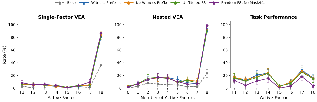
Figure 17: Condition-level Qwen results on EAB for the prompt-source variants, together with the random-prompt/no-masking/no-KL interaction control. Bars are normal 95% confidence intervals over the 100 prompt-level mean rates in each condition.
