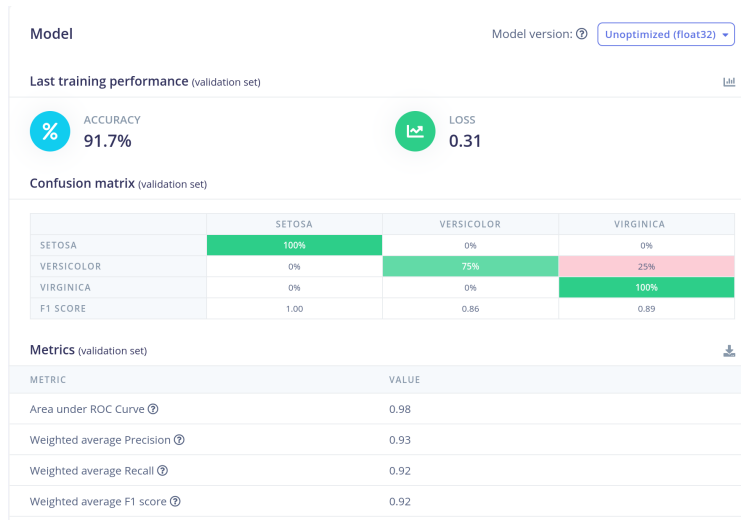
Figure 1: Training accuracy for the default model.
