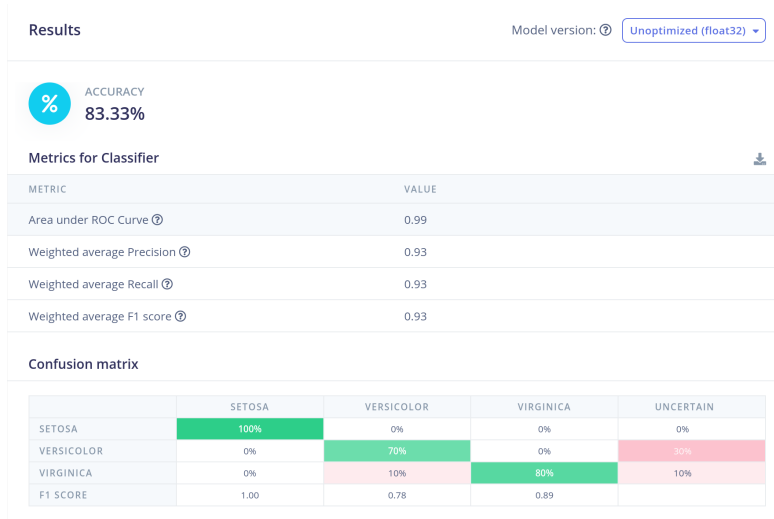
Figure 2: Testing accuracy for the default model.
