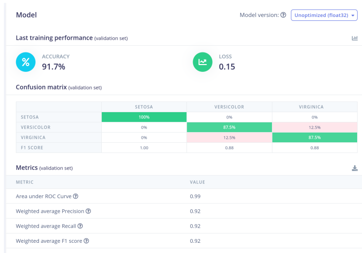
Figure 4: Training accuracy for the new model.
