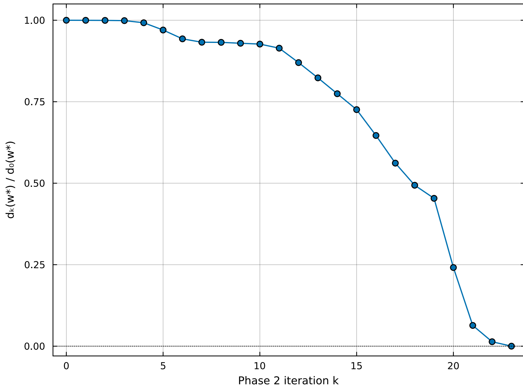
(b) Monotone projection-error decrease (Cor. 1)
