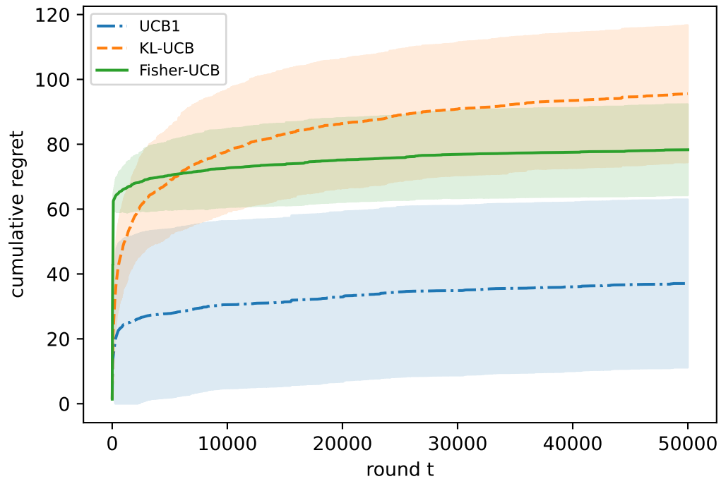
Binomial favorable ( \rho < 0, p < 1/2 )
