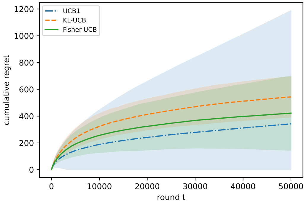
Poisson, small gaps (best=2.2, gaps 0.1-0.3)
