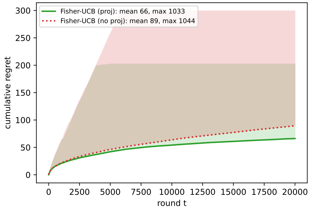
Poisson near zero (best=0.20): role of projection
