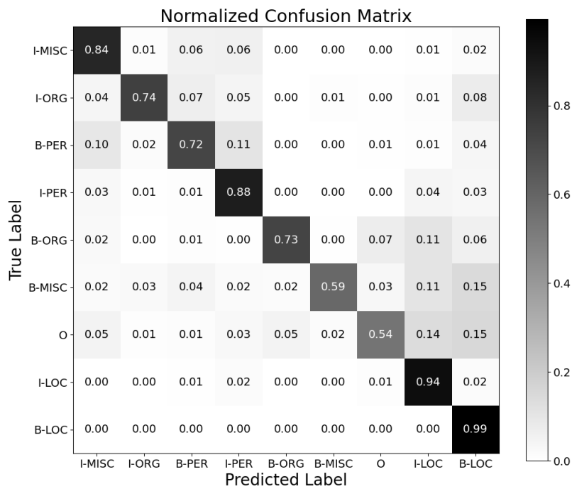
Figure 12: Confusion matrix for SVM tuned.
