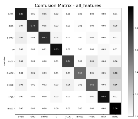
Figure 4: Confusion matrix for Linear SVM model with all features.
