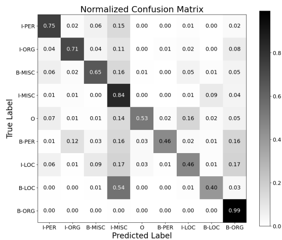
Figure 3: Confusion matrix of the Logistic Regression model on the development set.
