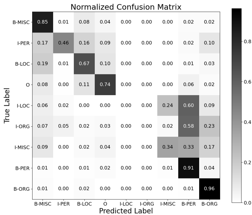
Figure 11: Confusion matrix for Naive Bayes model.
