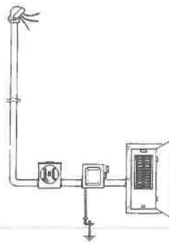
Temporary Electrical Service
