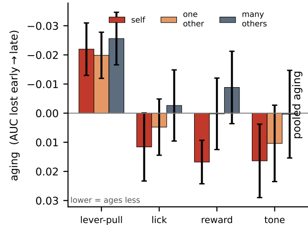
Count-matched: whose data ages less? (equal training-event count, sessions held out)
