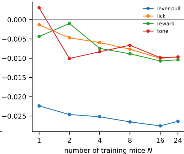
Scaling with training-set diversity
