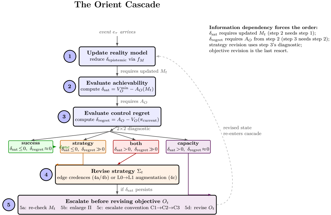
Figure 5: The orient cascade: a five-step resolution order forced by information dependency, not design. The 2x2 diagnostic at step 3 routes the agent to revise the strategy, to escalate before revising the objective, or to terminate at success or capacity limit; a revised model re-enters at step 1.
