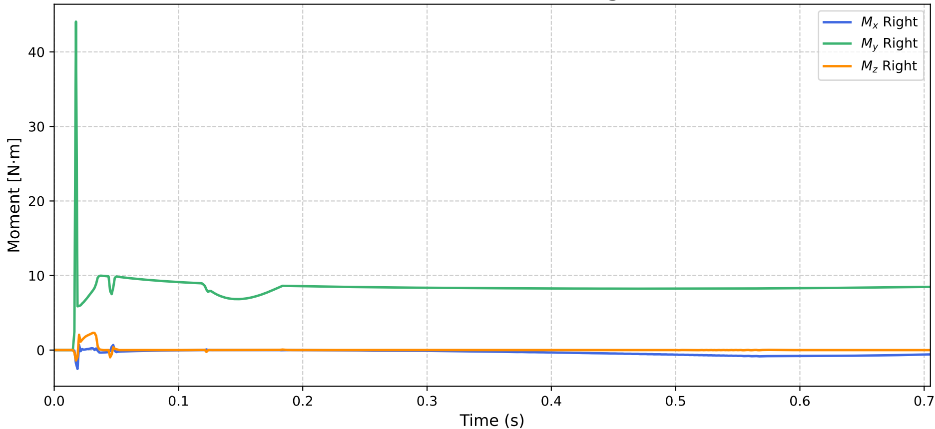
Ground Reaction Moment – Right Foot
