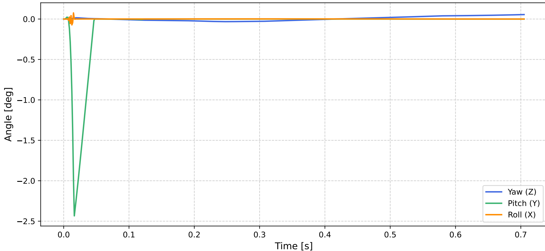
Left Foot Orientation (Euler ZYX)
