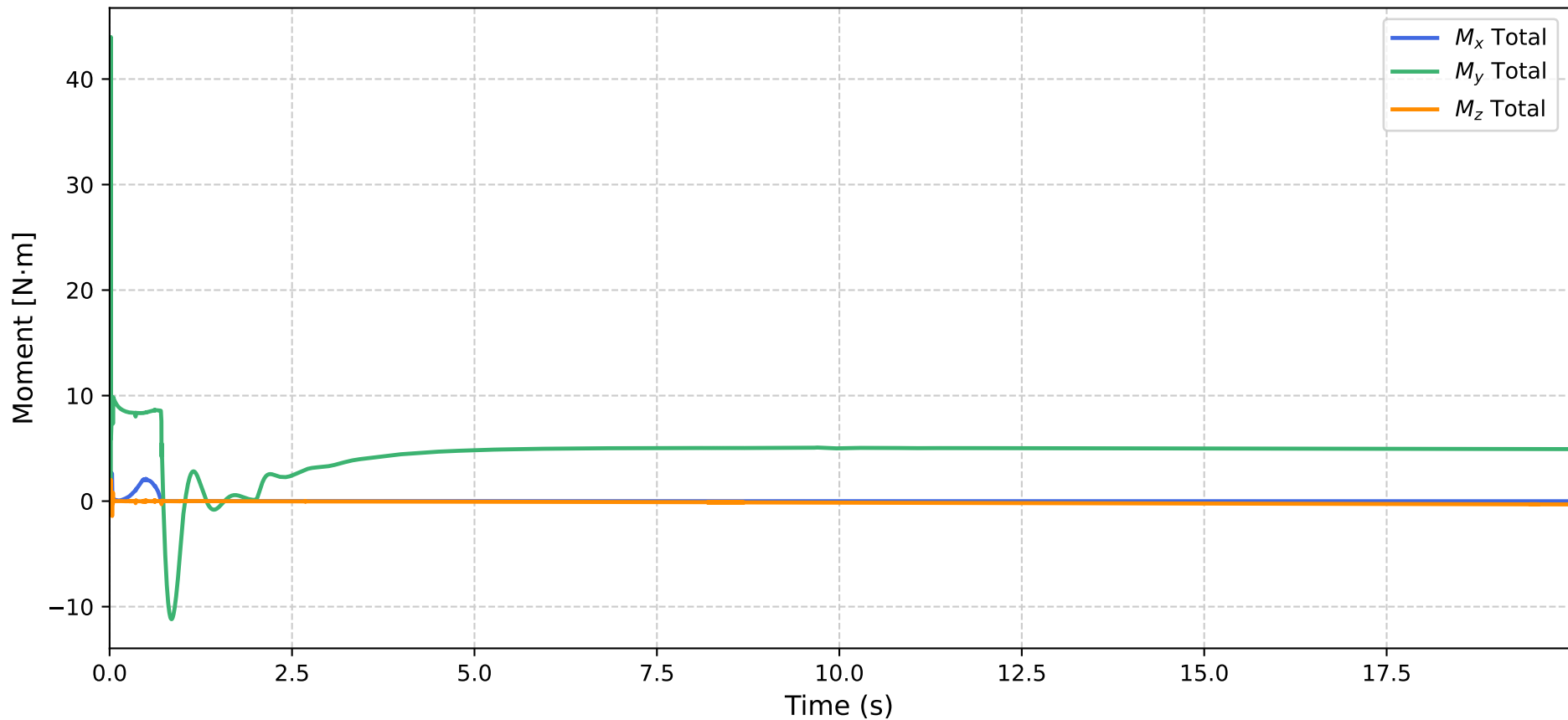
Total Ground Reaction Moment – Left Foot
