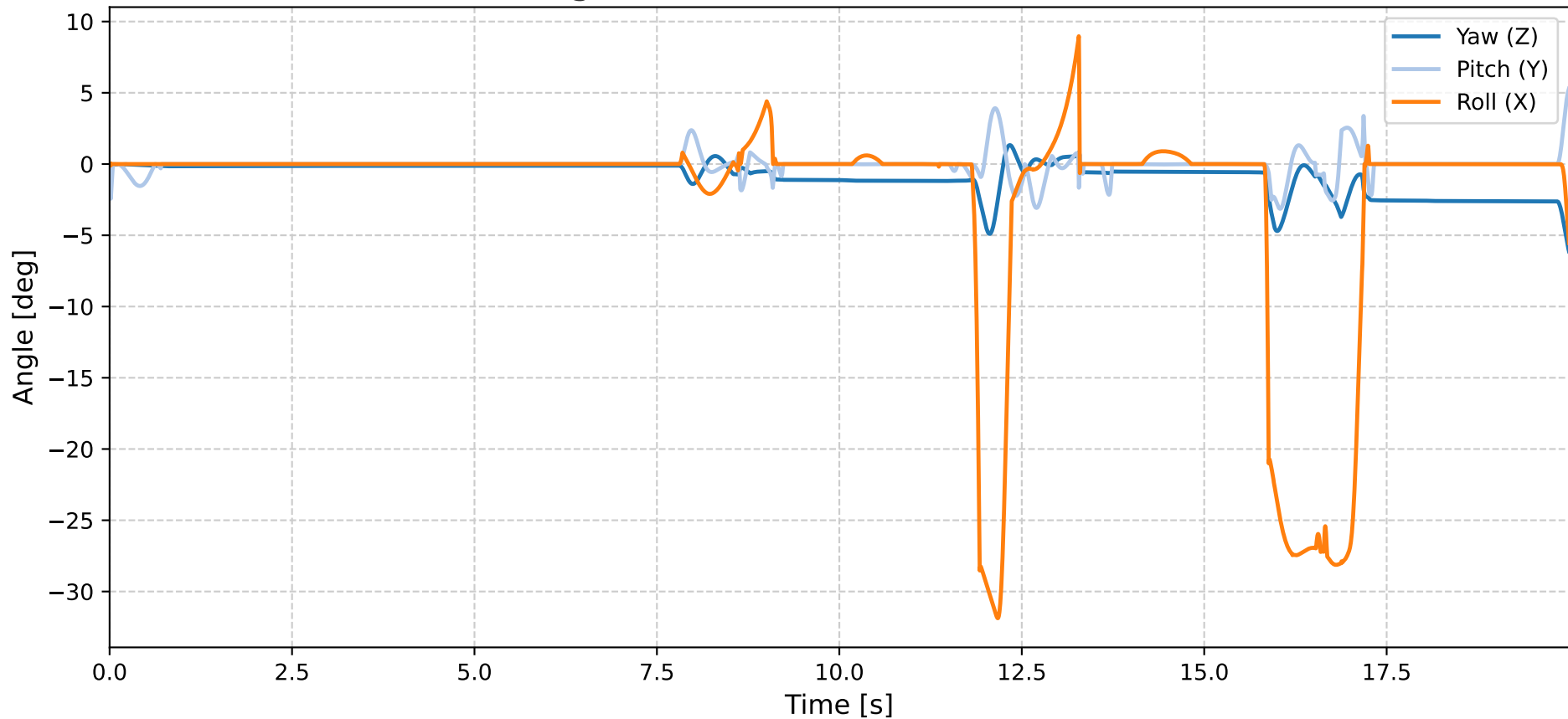
Right Foot Orientation (Euler ZYX)
